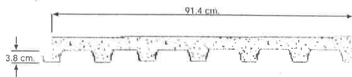
DECK 15T/36
